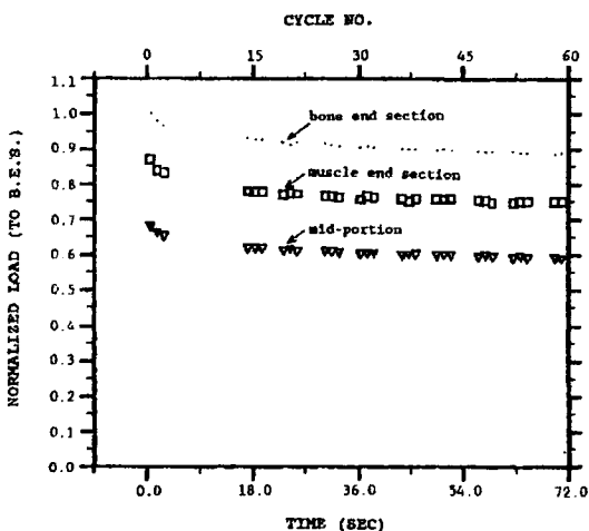
Fig. 3 Normalized load responses to the first peak load of the bone end section for the bone end section (test no. 1), mid-portion (test no. 2), and muscle end section (test no. 3) form a tendon of peroneous longus with the first sixty cycles
