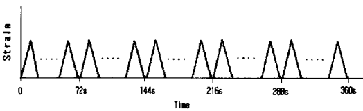
(a) Constant peak strain level test (A-type)
