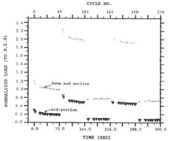
Fig. 7 Normalized load responses to the first peak load of the bone end section for the bone end section (test no. 6) and mid-portion (test no. 7) from a tendon of flexor digitorum longus at the C-type test
